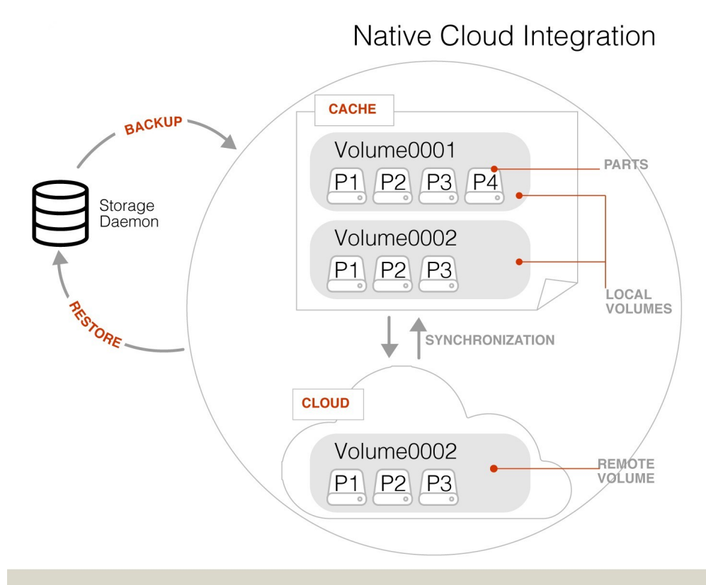
Figure 2.1: Bacula Cloud Architecture
