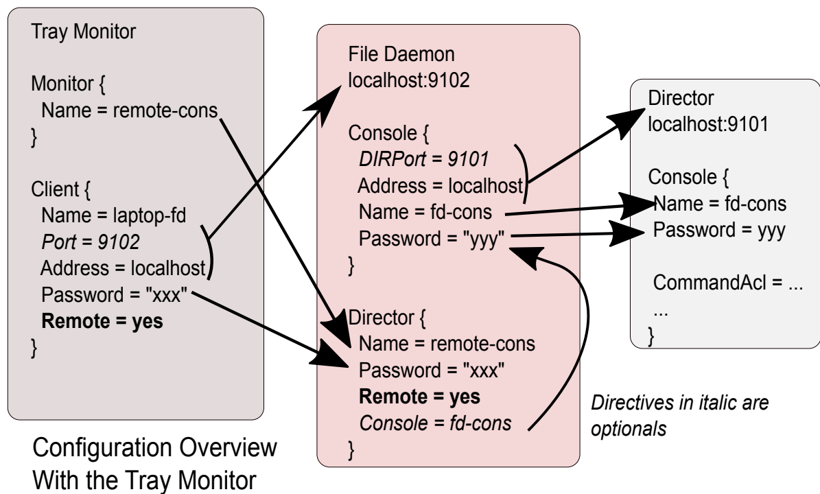
Figure 4.4: Relation Between Resources (tray-monitor)
