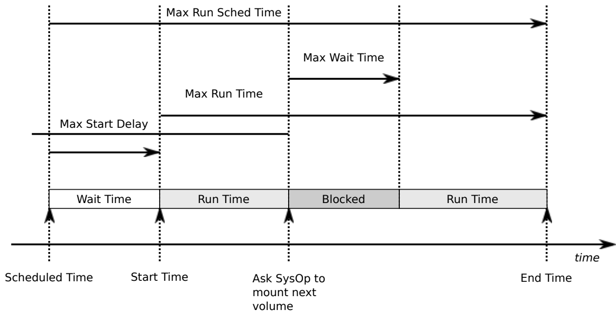
Figure 19.1: Job time control directives
