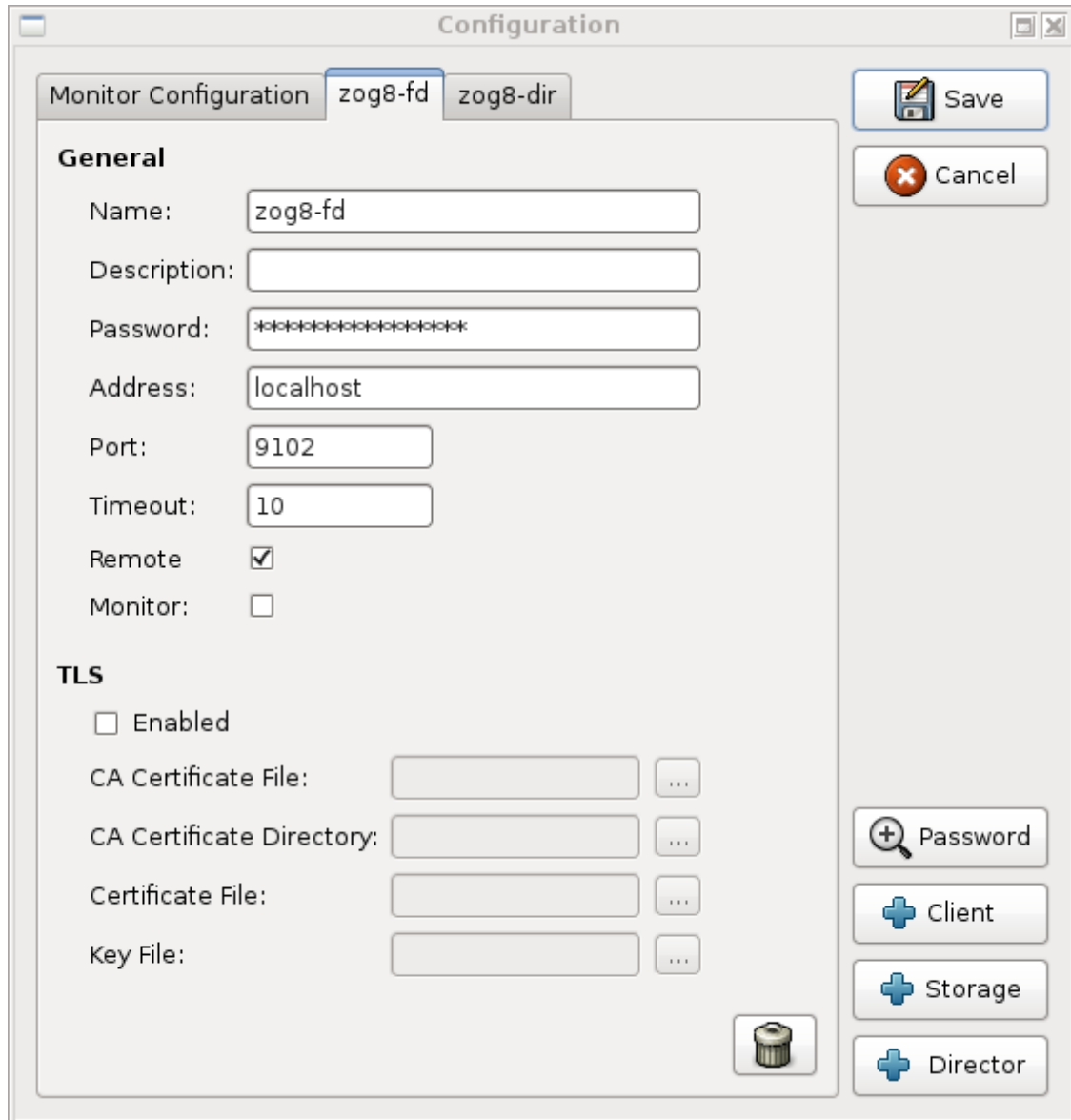
Figure 4.6: Tray Monitor Client Configuration
