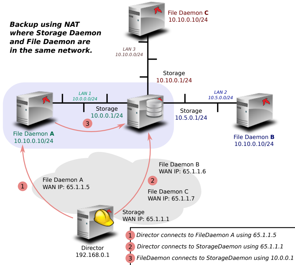
Figure 19.3: Backup over WAN using FD Storage Address
