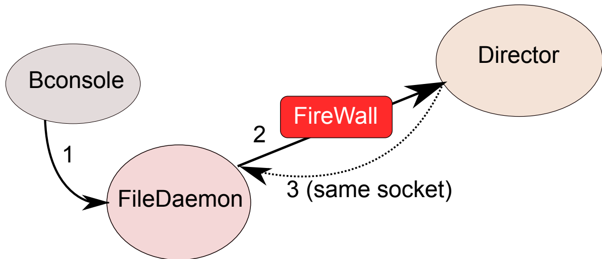
Figure 4.2: Client Initiated Backup Network Flow
