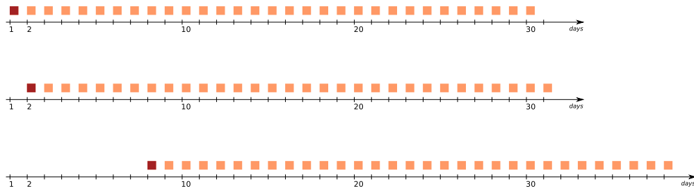
Figure 4.1: Backup Sequence Slides Forward One Day, Each Day
