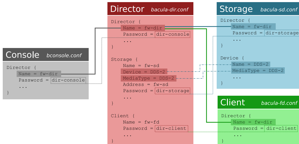
Figure 21.2: Configuration diagram
